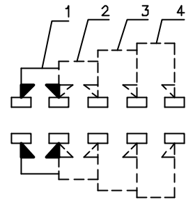
NON-SHORTING SCHEMATIC
