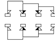
NON-SHORTING SCHEMATIC
