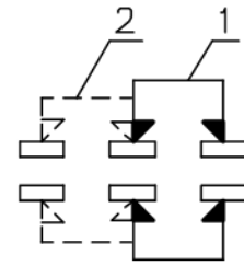
NON-SHORTING SCHEMATIC
