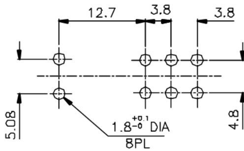
PRINTED CIRCUIT PANEL LAYOUT
