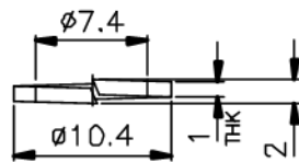
SPRING WASHER
