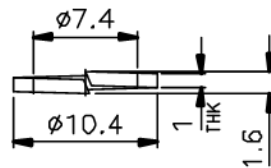
SPRING WASHER
