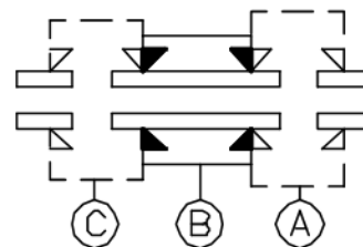
NON-SHORTING SCHEMATIC
