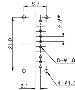
PC MOUNTING
