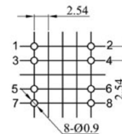
Circuit Diagram PCB HOLE( BOTTOM VIEW)
