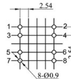
Circuit Diagram PCB HOLE( BOTTOM VIEW)
