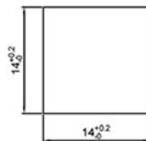
PANEL HOLE
