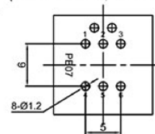
PCB HOLE (BOTTOM VIEW)
