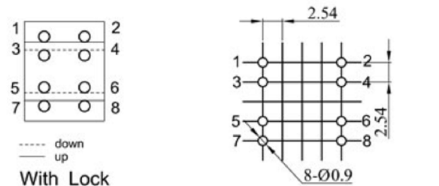
Circuit Diagram PCB HOLE( BOTTOM VIEW)
