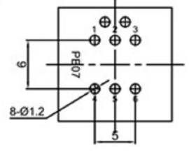
PCB HOLE(BOTTOM VIEW)
