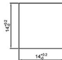
PANEL HOLE
