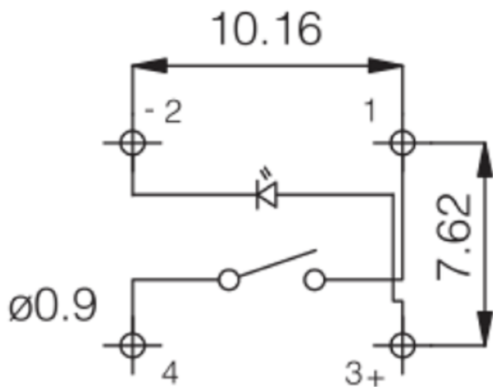
CIRCUIT
