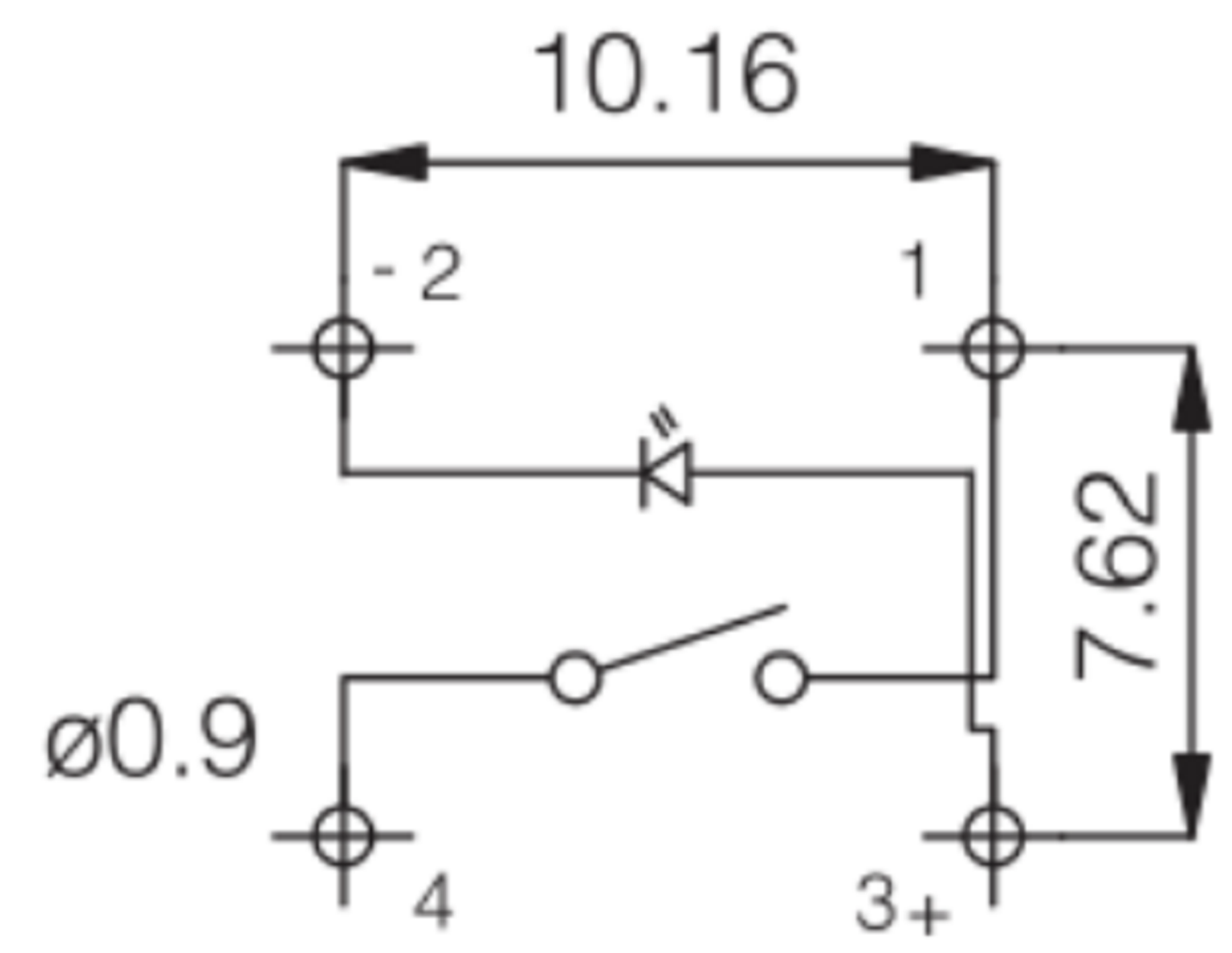
CIRCUIT
