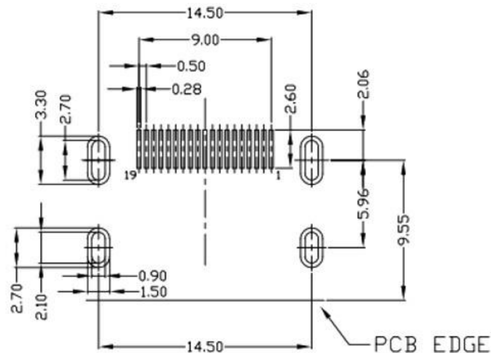
RECOMMENDED PCB LAYOUT (T=1.60mm)
