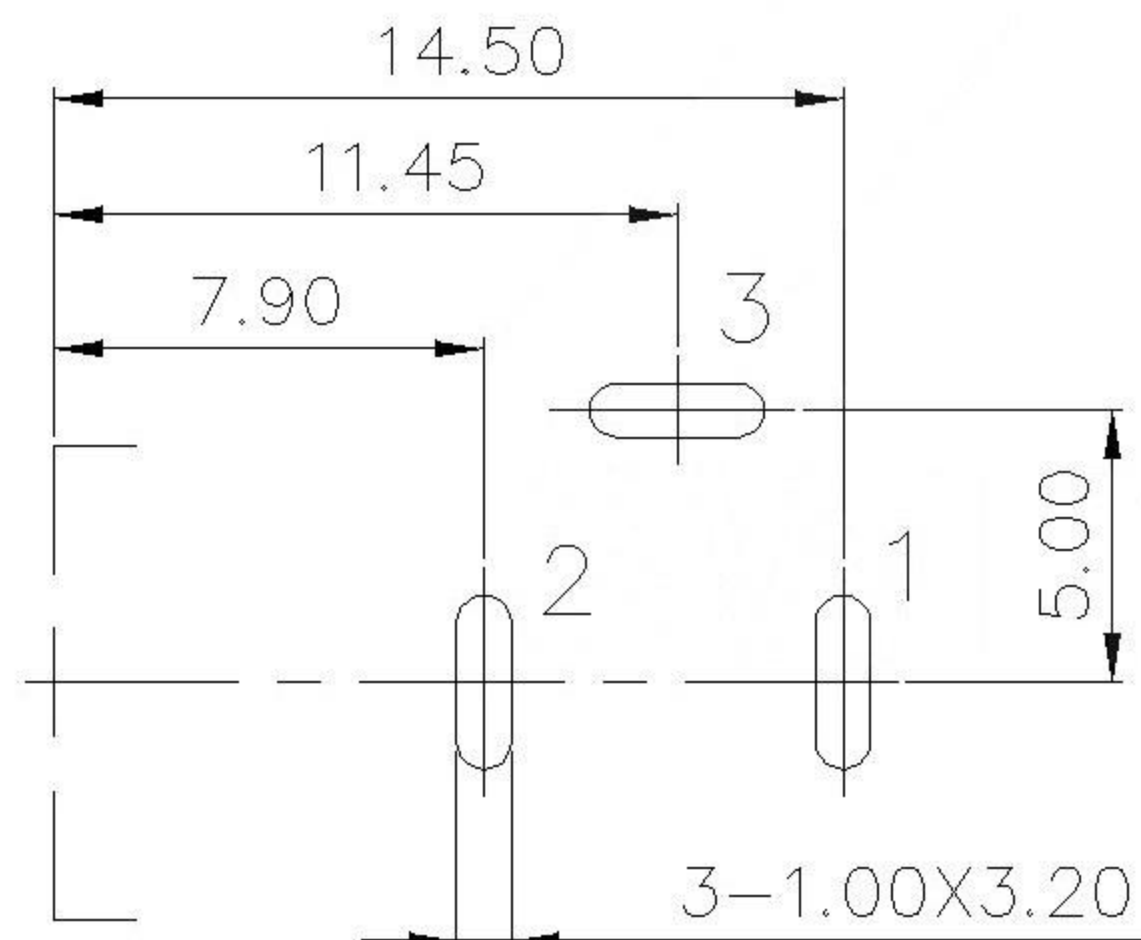
Pin Hole Layout (Jack Bottom View)
