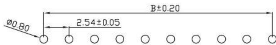
PCB LAYOUT
