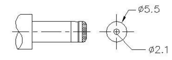
MATING PLUG Jack Insertion Depth: 9.15 mm
