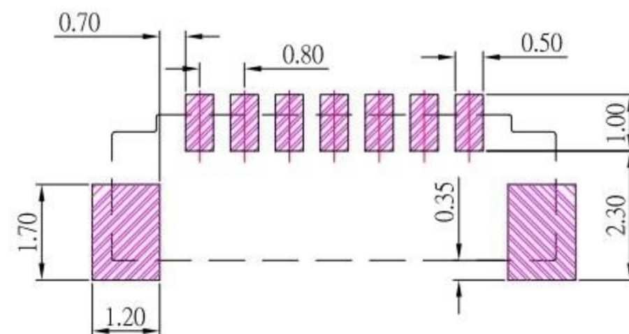
P.C.B LAYOUT MOUNTING PATTERN
