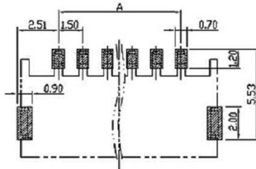
Recommended P.C.Board Layout (top view)
