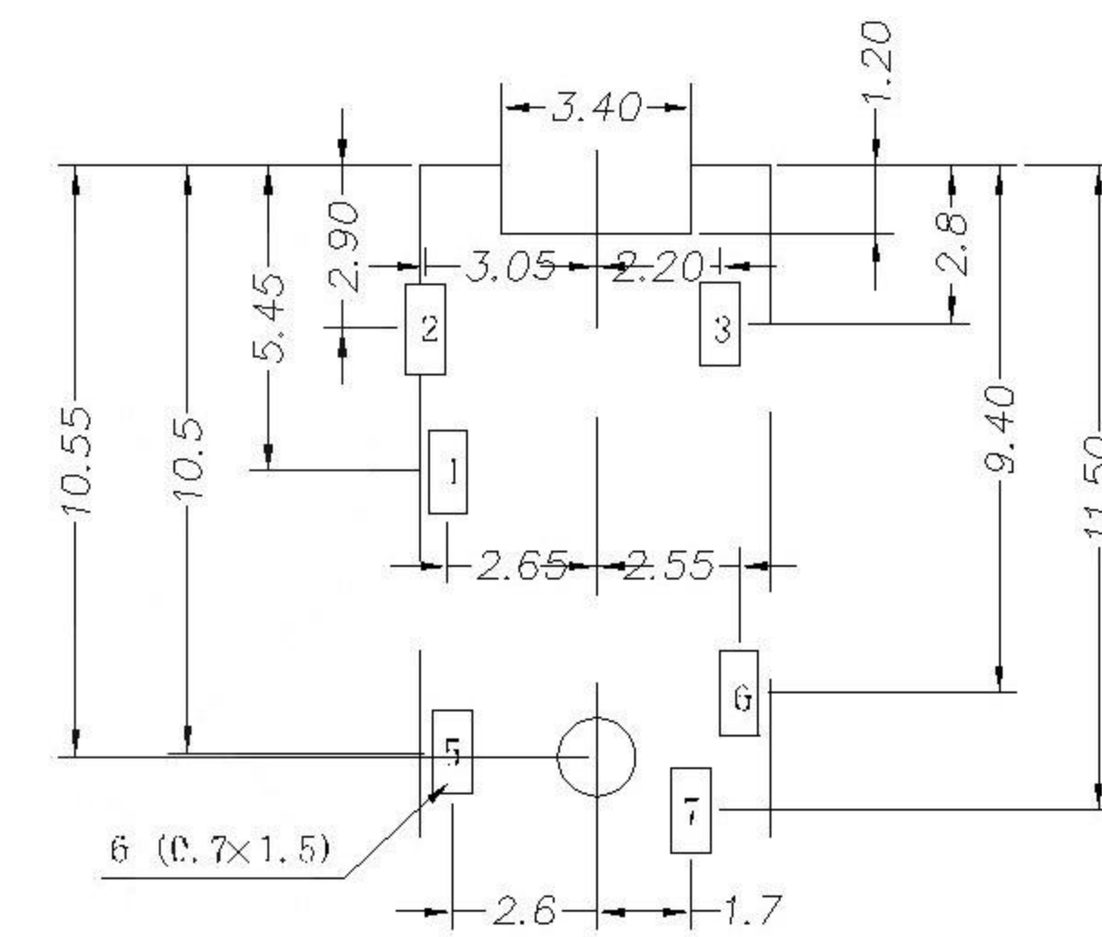
P. C. B LAYOUT TOP VIEW
