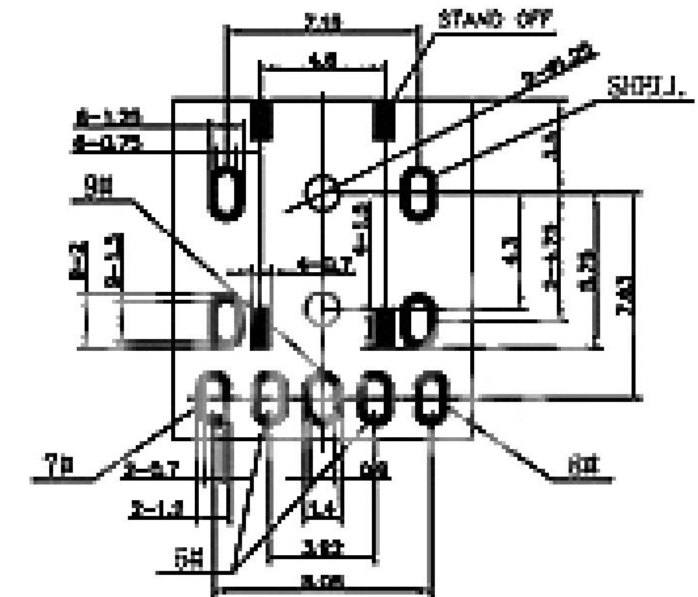
PCB LAYOUT TOP VIEW (Tolerance:±0.05)
