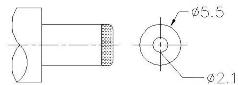
MATING PLUG Jack Insertion Depth: 9.0 mm
