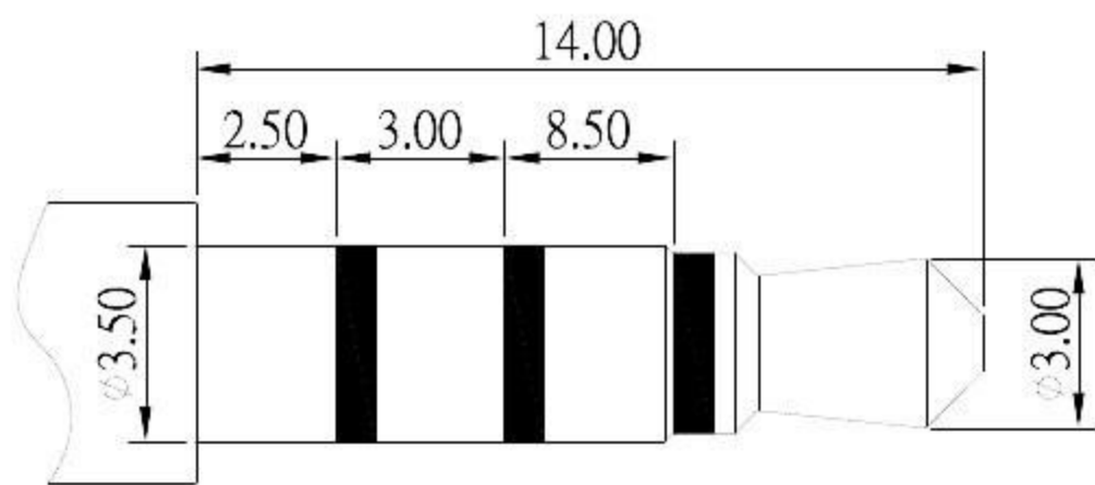
Ø3.50mm 4 POLE PLUG
