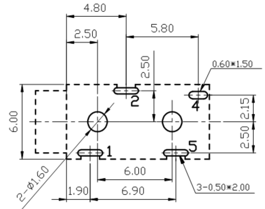
Pin Hole Layout (Jack Bottom View)
