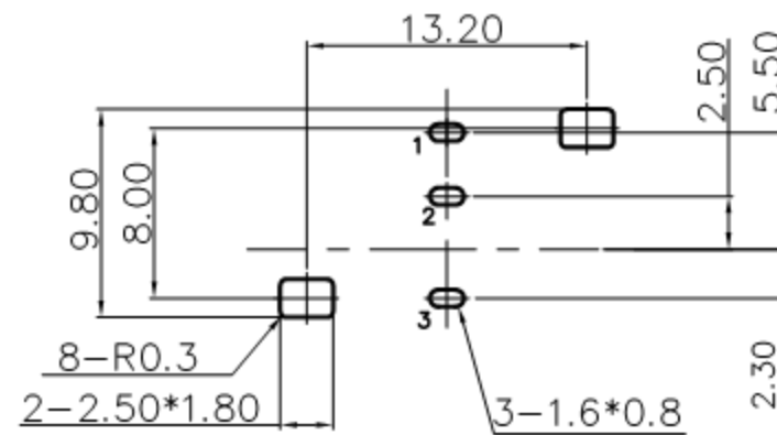
Pin Hole Layout (Jack Bottom View)
