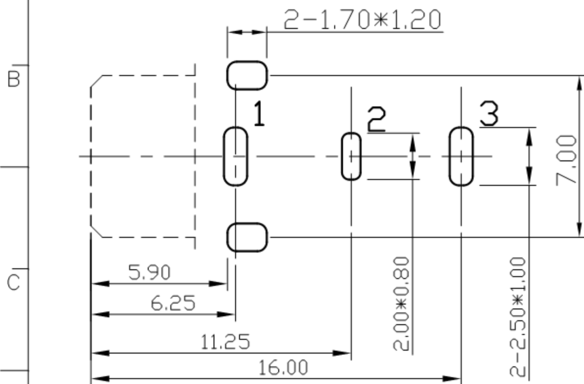
Pin Hole Layout Jack Bottom View
