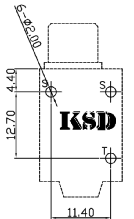
Pin Hole Layout (Jack Bottom View)
