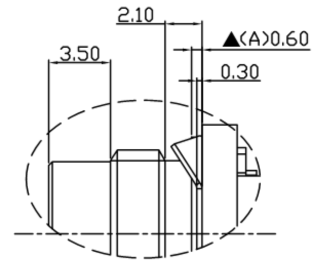
"A" Detail
