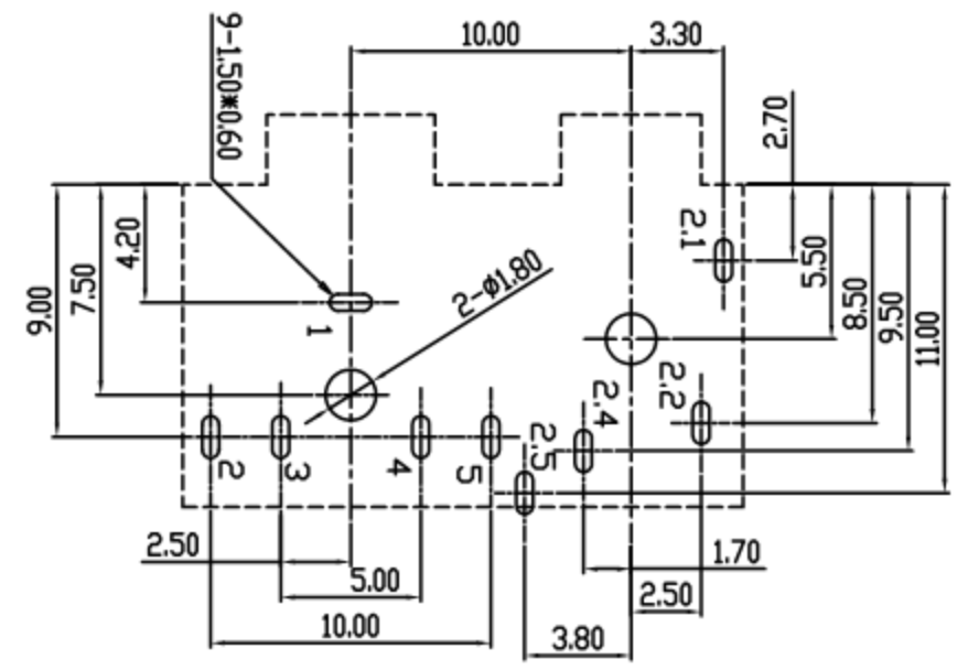
Pin Hole Layout (Jack Bottom View)
