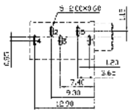
Pin Hole Layout (Jack Bottom View)
