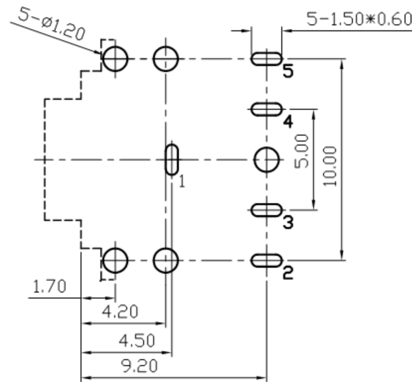
Pin Hole Layout (Jack Bottom View)
