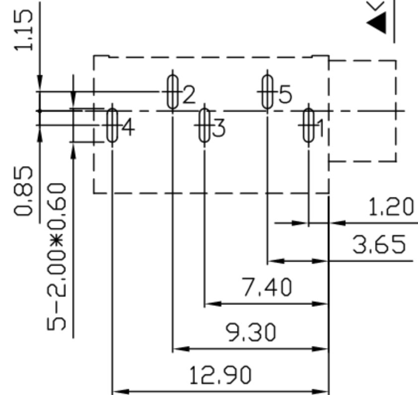
Pin Hole Layout (Jack Bottom View)
