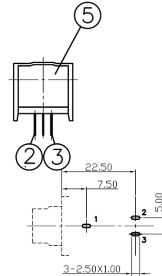
Pin Hole Layout (Jack Bottom View)
