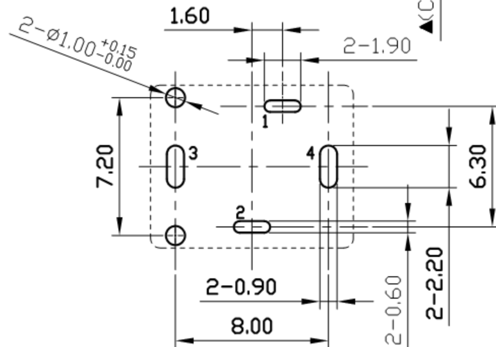
Pin Hole Layout (Jack Bottom View)
