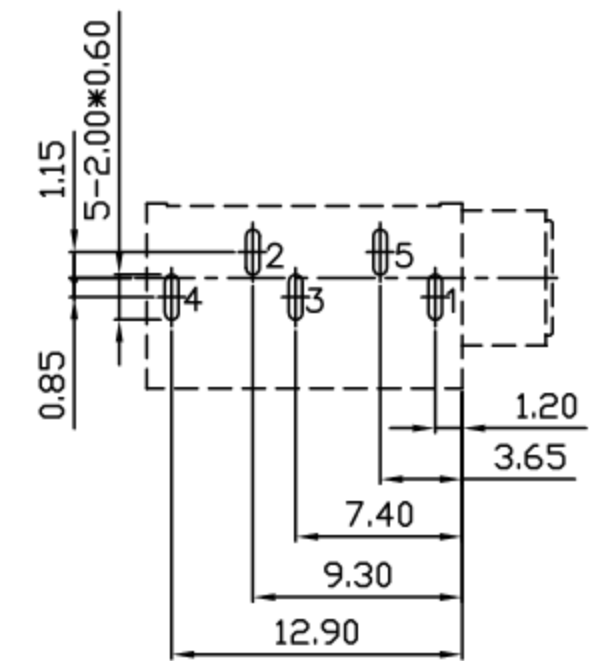
Pin Hole Layout (Jack Bottom View)
