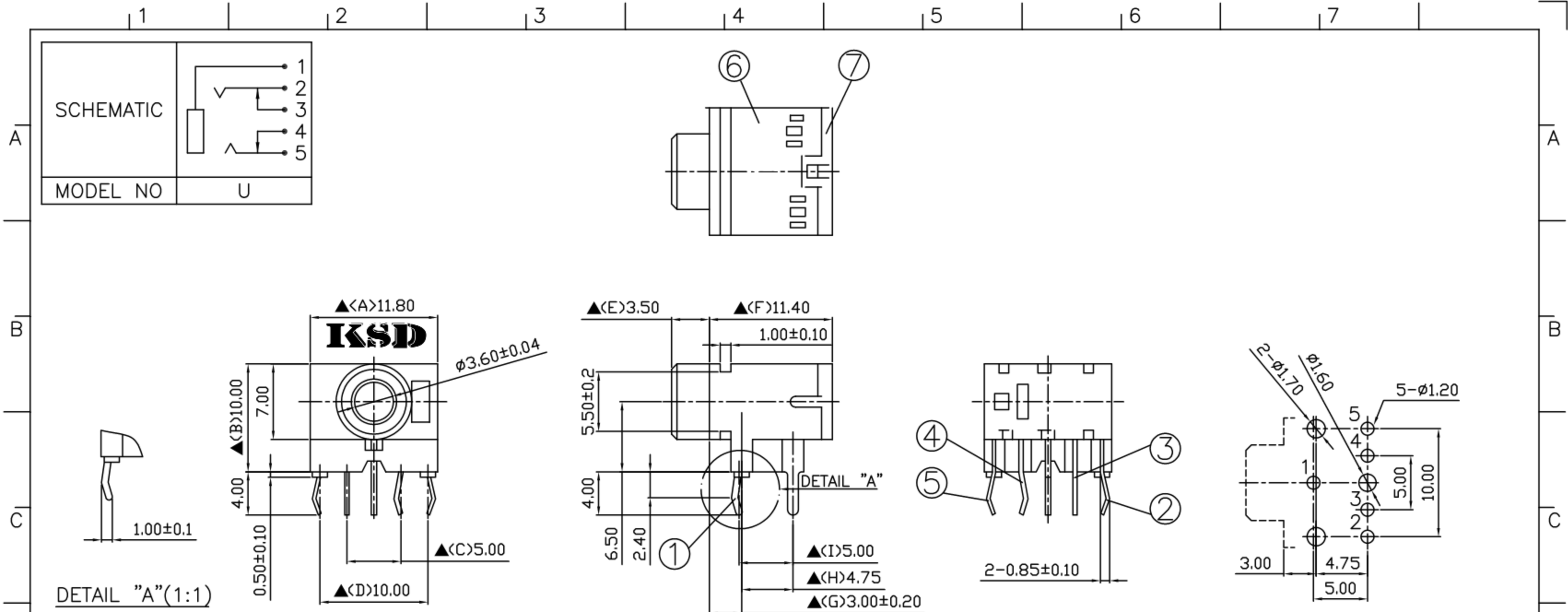
Pin Hole Layout (Jack Bottom View)
