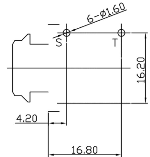
Pin Hole Layout (Jack Bottom View)
