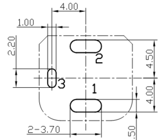
Pin Hole Layout (Jack Bottom View)
