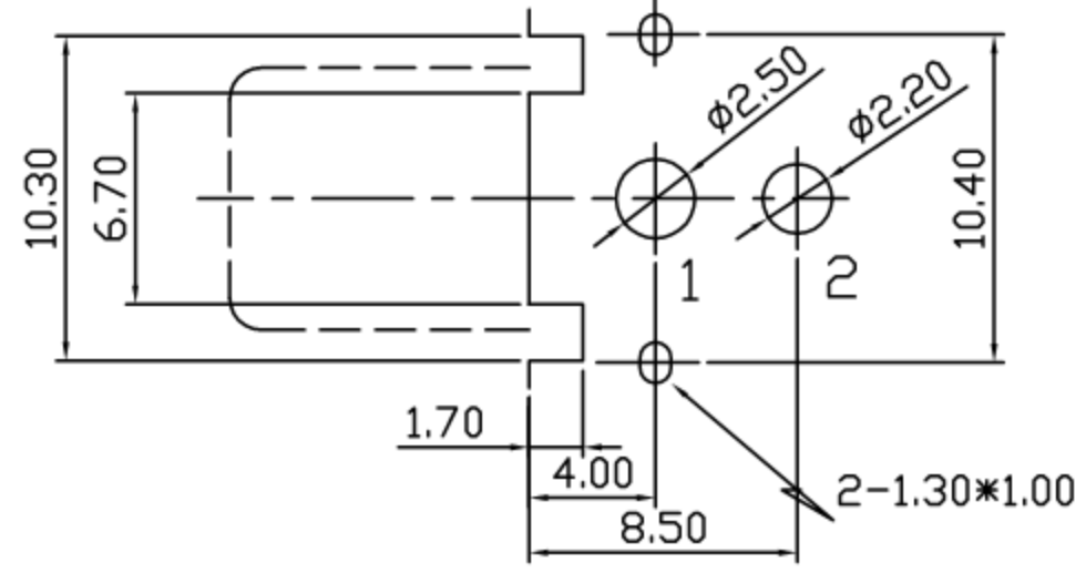
Pin Hole Layout (Jack Bottom View)
