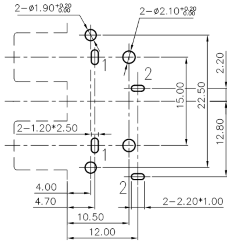
Pin Hole Layout (Jack Bottom View)
