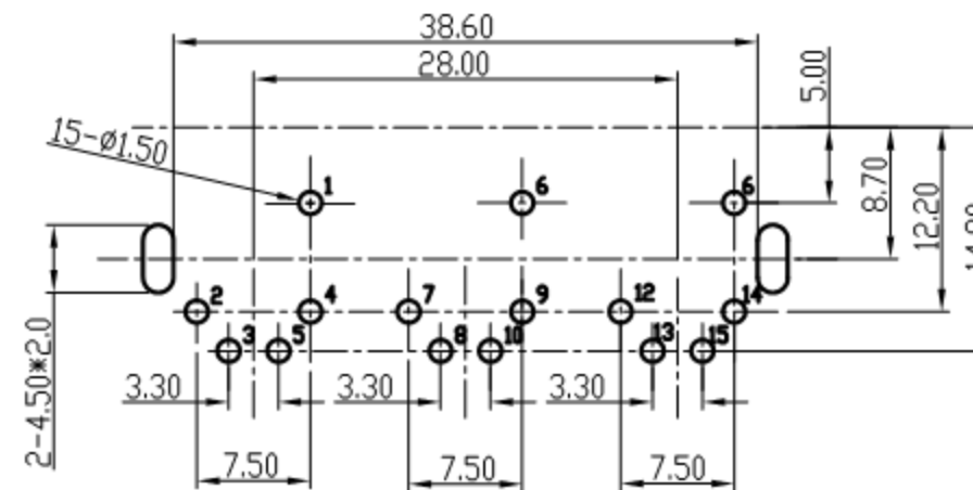
Pin Hole Layout (Jack Bottom View)
