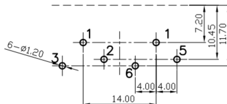
Pin Hole Layout (Jack Bottom View)
