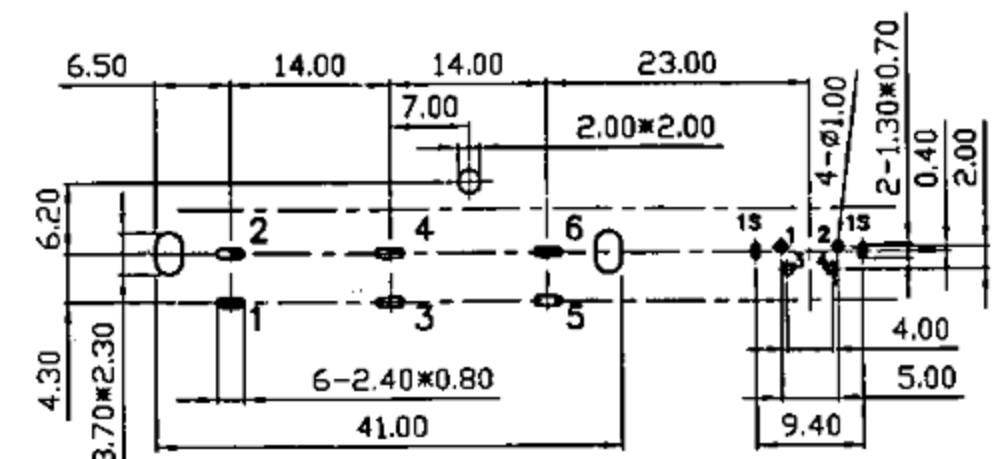
Pin Hole Layout (Jack Bottom View)
