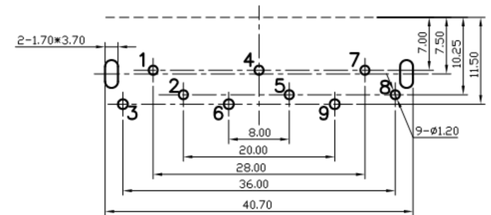
Pin Hole Layout (Jack Bottom View)
