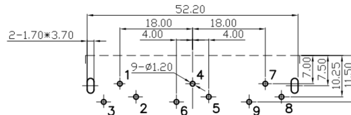
Pin Hole Layout (Jack Bottom View)
