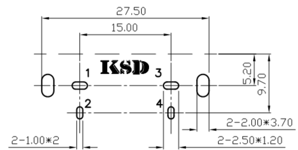
Pin Hole Layout (Jack Bottom View)
