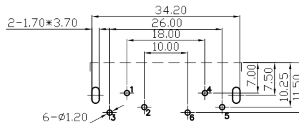
Pin Hole Layout (Jack Bottom View)
